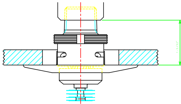
Standard Installation
