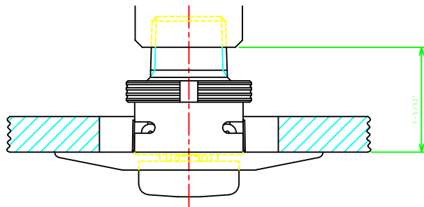
Standard Installation
