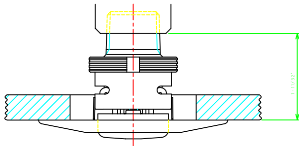
Flush Minimum
