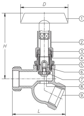
1/2" FIP
