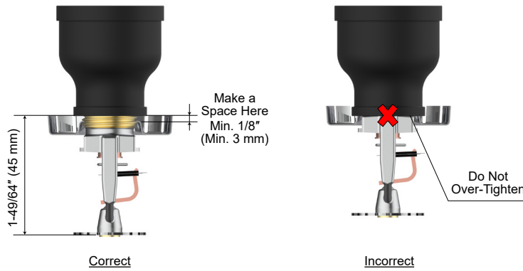
Figure 4: Installation (Correct and Incorrect)
