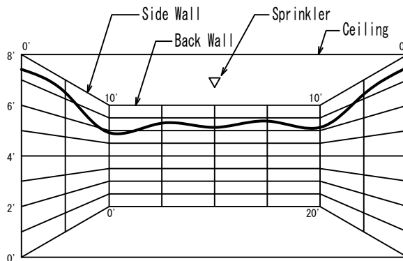
SS4451 FR-RES 4.9K 20GPM-16.7psi 20'x20' Room Size (Half Pattern)
