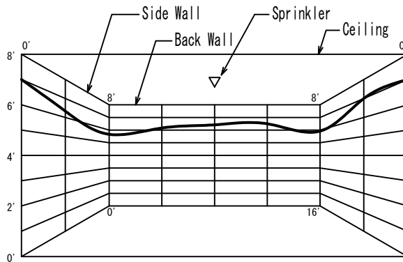
SS4451 FR-RES 4.9K 14GPM-8.2psi 16'x16' Room Size (Half Pattern)
