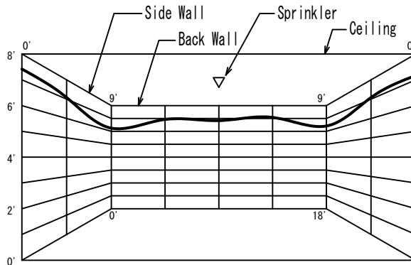
SS4451 FR-RES 4.9K 17GPM-12.0psi 18'x18' Room Size (Half Pattern)
