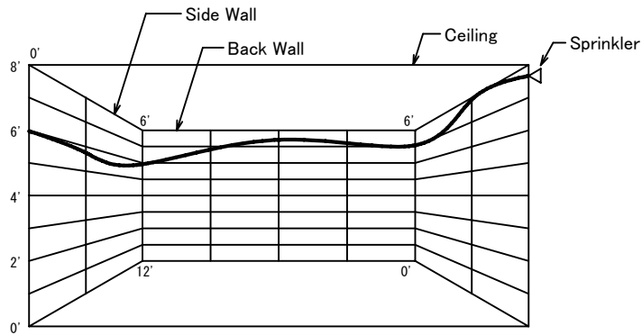
SS4423 HF-RES 4.2K 13GPM-9.6psi 12'x12' Room Size (Half Pattern)
