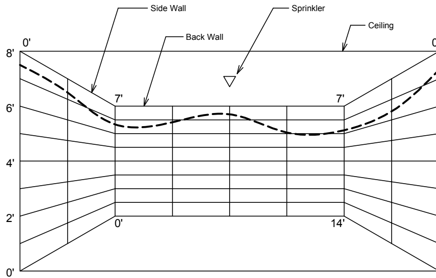
SS8261 RC-RES 3.7K 10GPM-7.3psi 14'x14' Room Size (Half Pattern)
