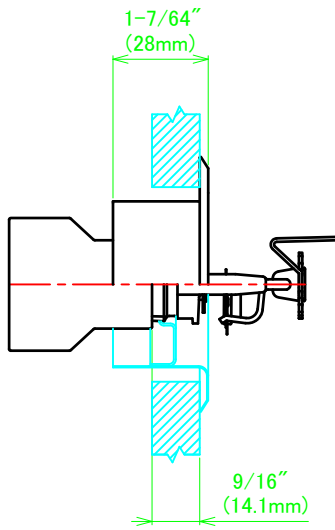
Standard Installation
