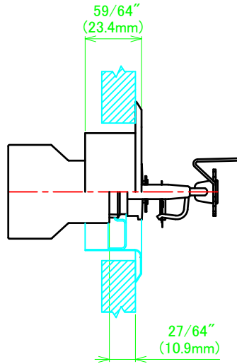
Standard Installation
